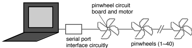
Figure 2 Setup of the Pinwheels system
